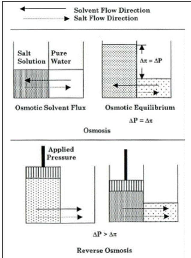
Figure 1. Reverse Osmosis vs. Osmosis
