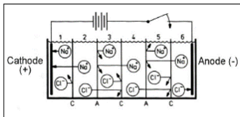
Figure 2. Electrodeionization Stack
